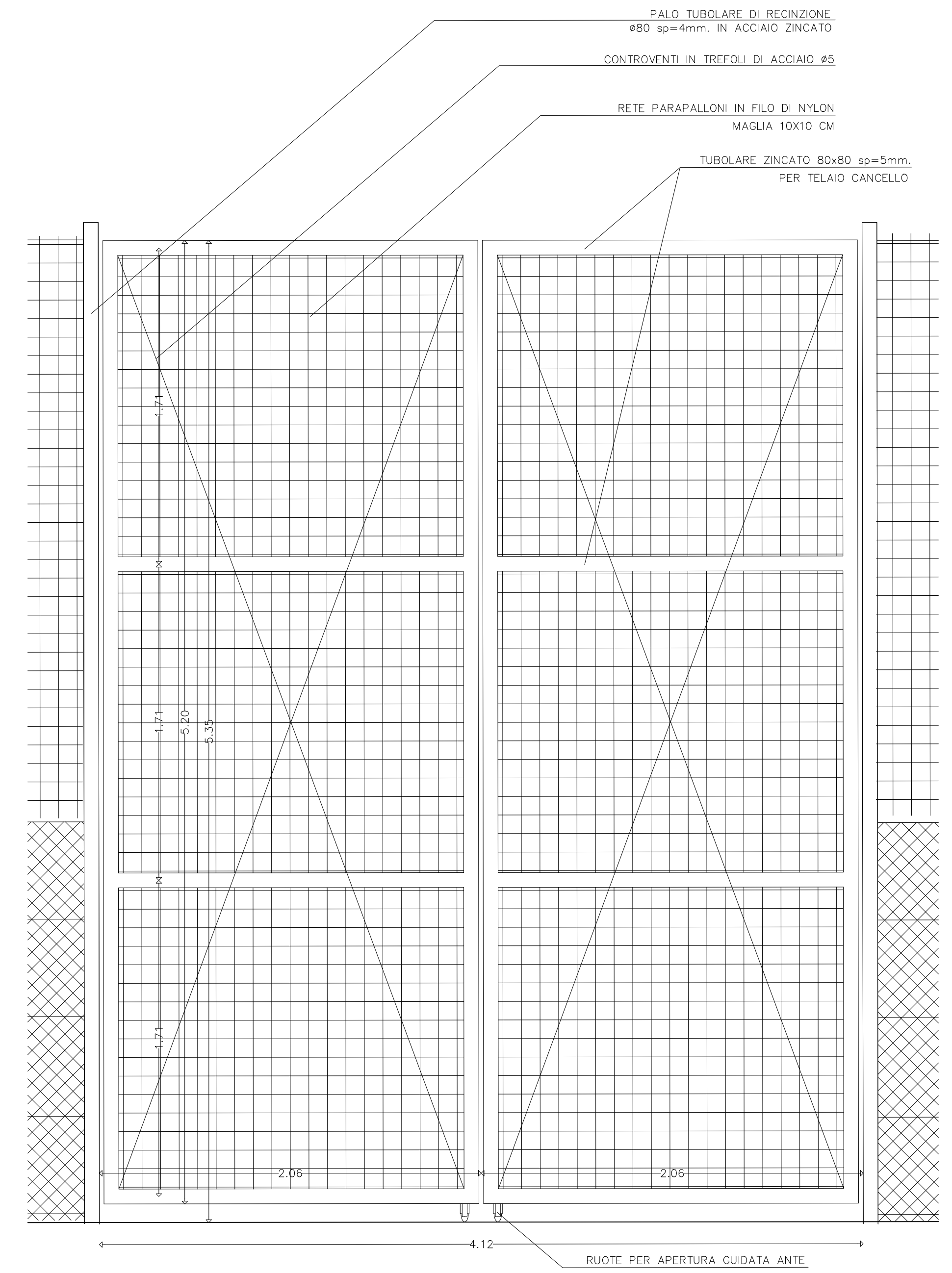
CANCELLO 412x535m DET. 01
